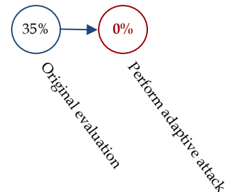
Robust Accuracy
