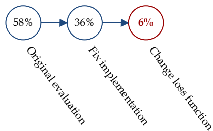
Robust Accuracy
