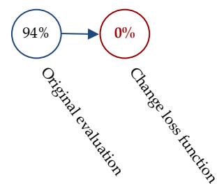
Robust Accuracy
