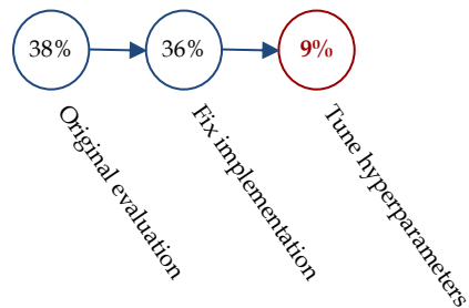
Robust Accuracy
